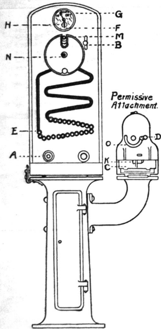
STAFF INSTRUMENT.
